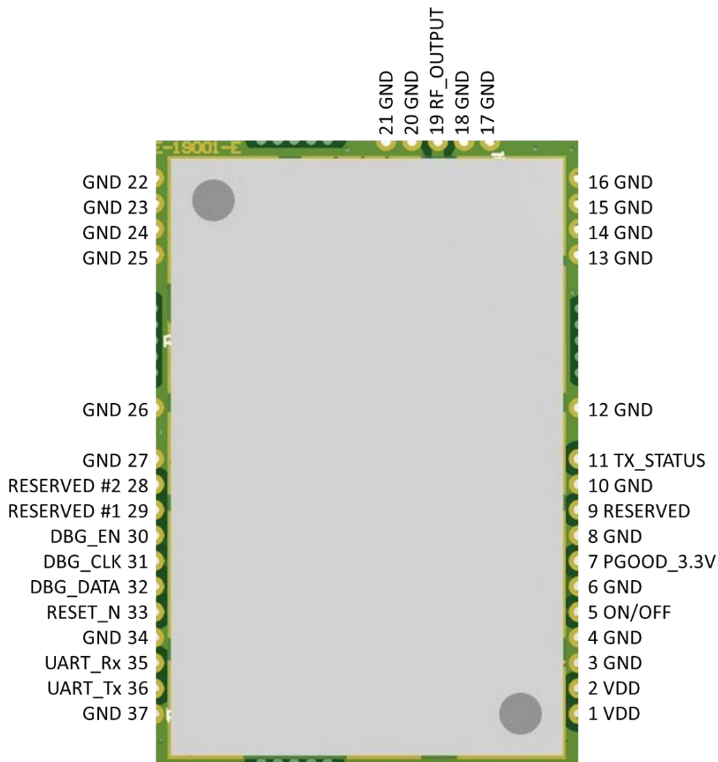
Figure 8: KIM1 pad assignments
