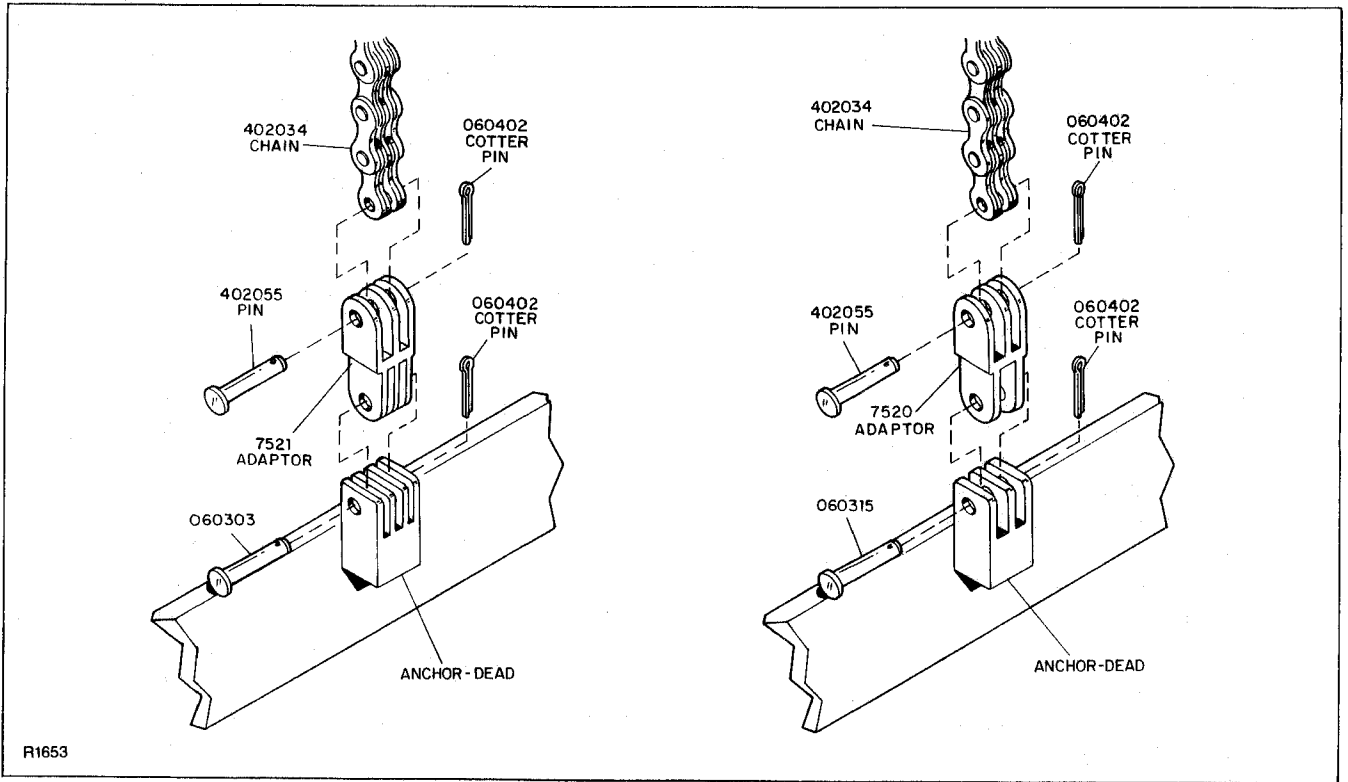
Figure 1. Typical Installation of Chain with Adaptor
