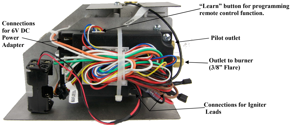
Figure 7 Pilot/Igniter Assembly
