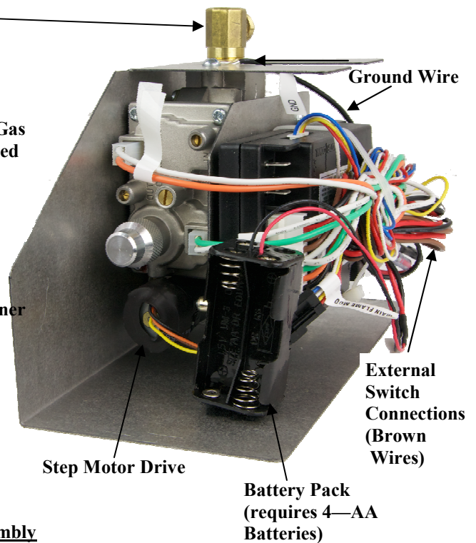
Figure 4—Front of Control Assembly
