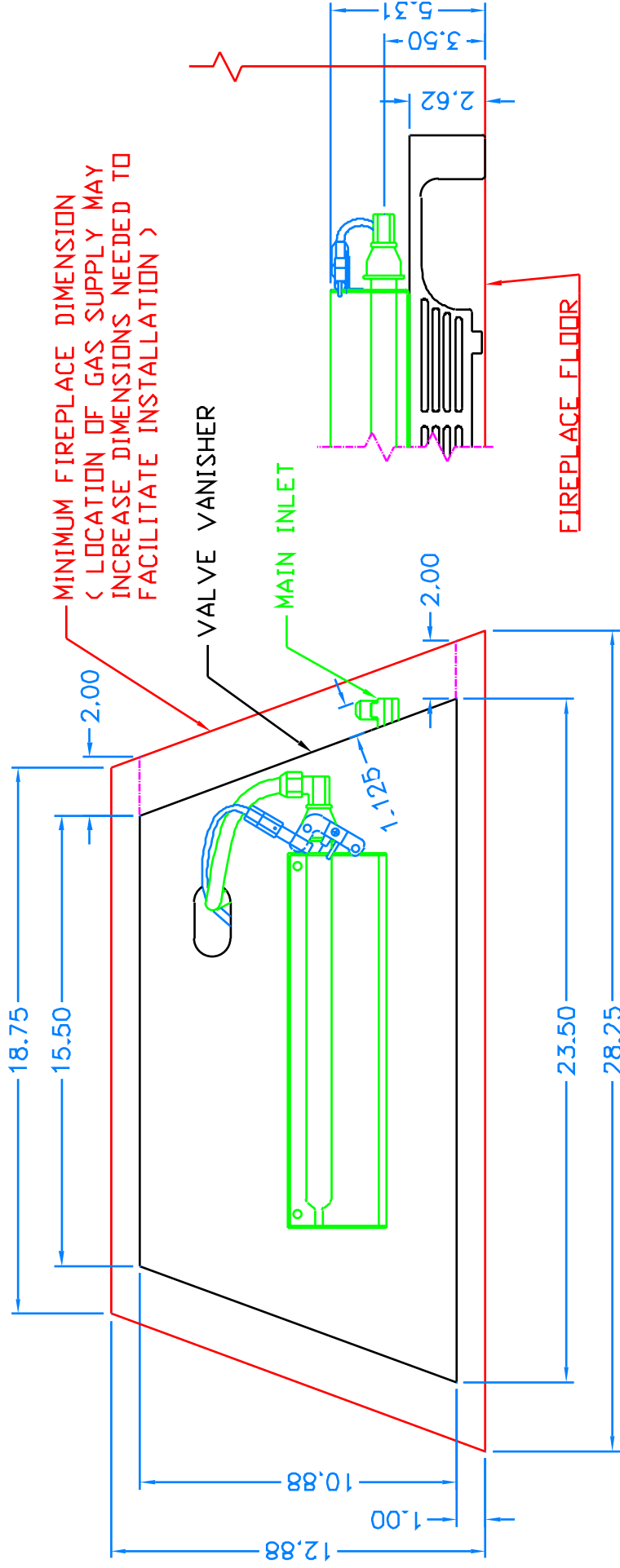
TOP VIEW
