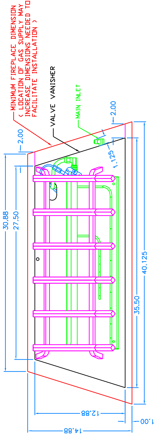
TOP VIEW
