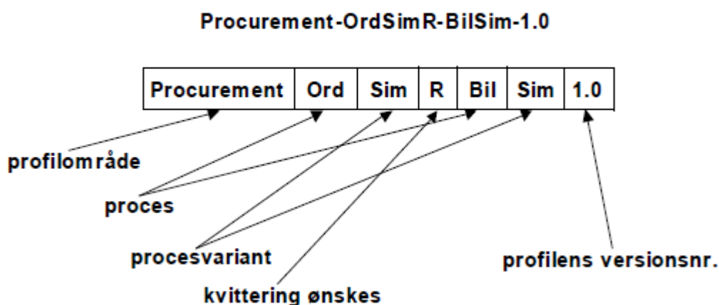
Figur 2: Procurement-OrdSimR-BILSIM-1.0
