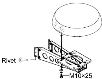
How to fasten the sensor to the radome mount
