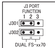
Detail for J301/302
