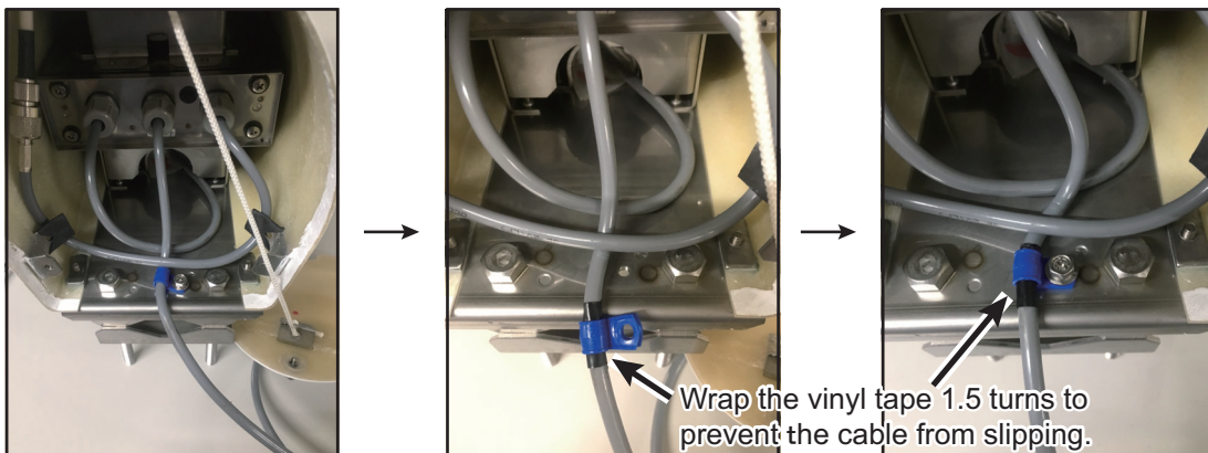
Installation overview of GPS/VHF combined antenna
