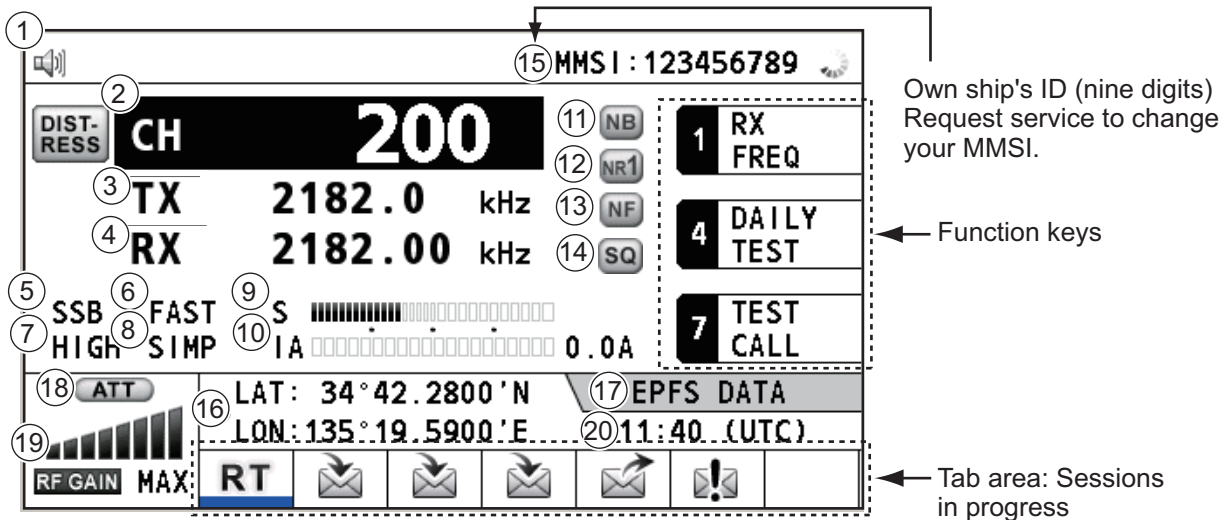
Radiotelephone (RT) screen
