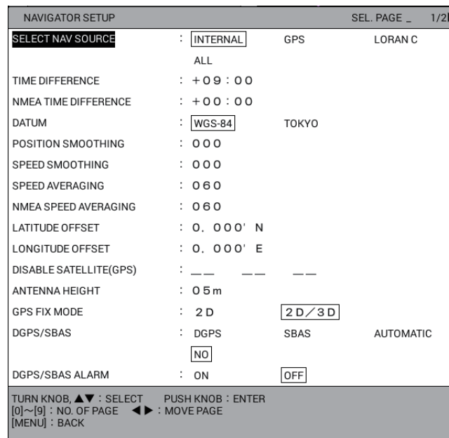
[NAVIGATOR SETUP] menu: Page 1
